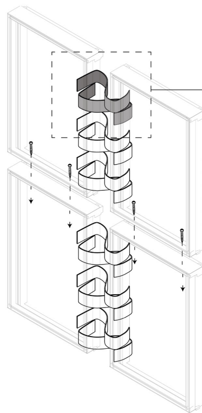
Axo showing the asseblly
