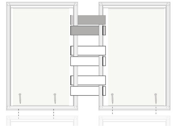
Elevation drawing 1:10
