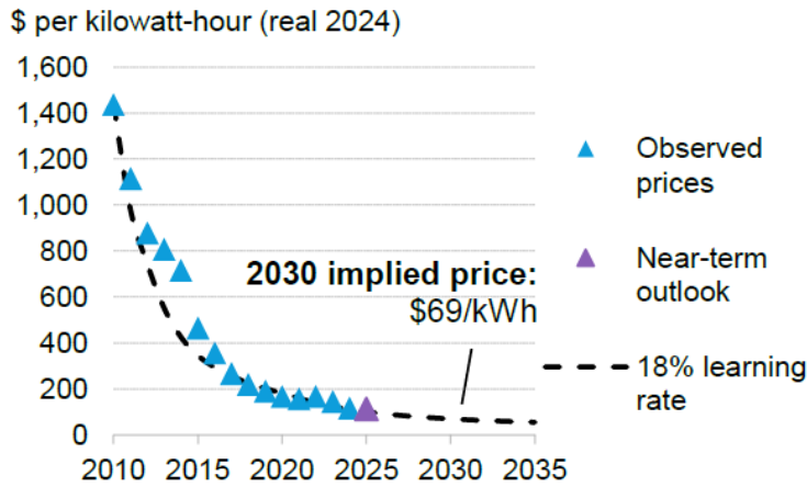
Figure 1: Lithium-ion battery pack price outlook
